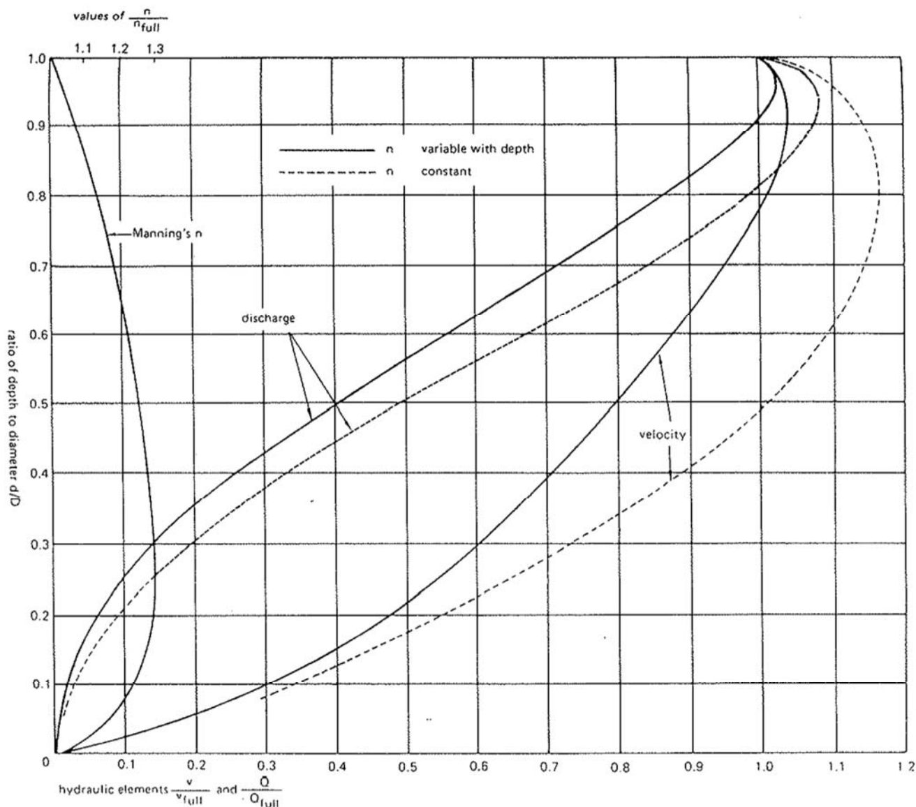
FIG. 1. Hydraulic Properties of Circular Sewers
